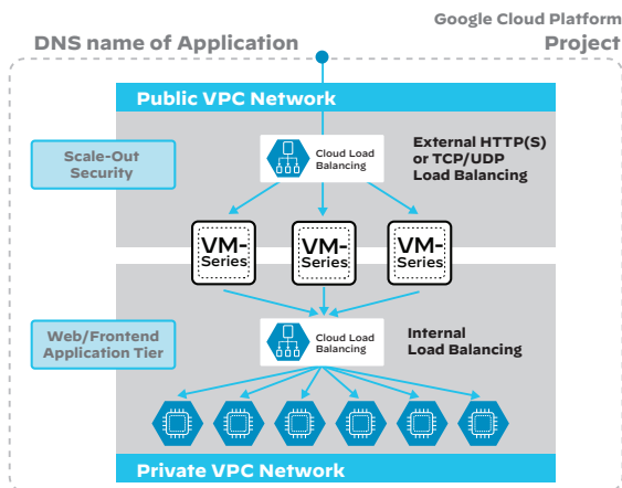
Figure 2: VM-Series scale-out architecture on GCP
